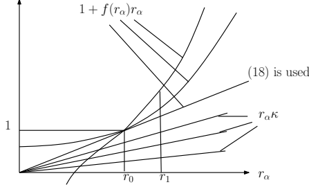
Fig. 3. Comparison of 1 + f(r_\alpha)r_\alpha and r_\alpha \kappa . Control law given by (21) is singular when \cos(\phi) = \frac{r_\alpha \kappa}{1 + f(r_\alpha)r_\alpha} . We argue that singular case can not be removed by choosing f(r_\alpha) if the curvature \kappa is upper bounded.
