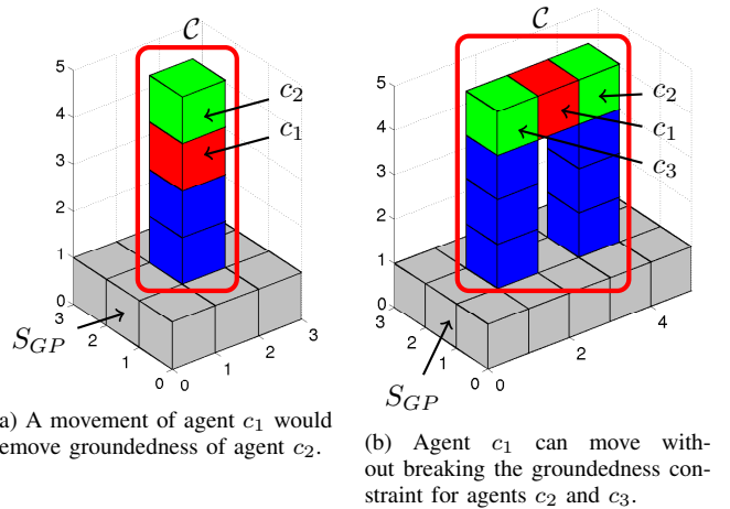
Fig. 2: Examples of grounded configurations and feasible motions of cubes.
