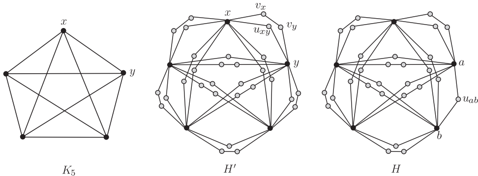
FIGURE 2. A complete graph K_5 . H' is obtained by replacing every edge xy \in E(K_5) , by disjoint paths xu_{xy}y and xv_x v_y y . H is obtained from H' , by deleting v_a and v_b , from two distinct vertices a and b . Note that every vertex of H that belongs to the original K_5 has degree 8, except a and b that have degree 7.
